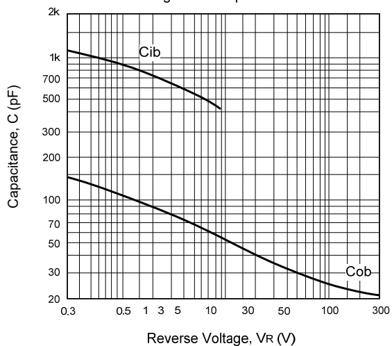
Figure 11. Capacitance
