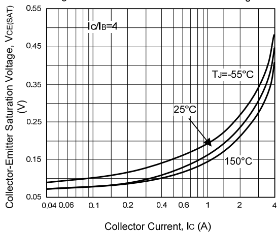
Figure 9. Collector-Emitter Saturation Voltage
